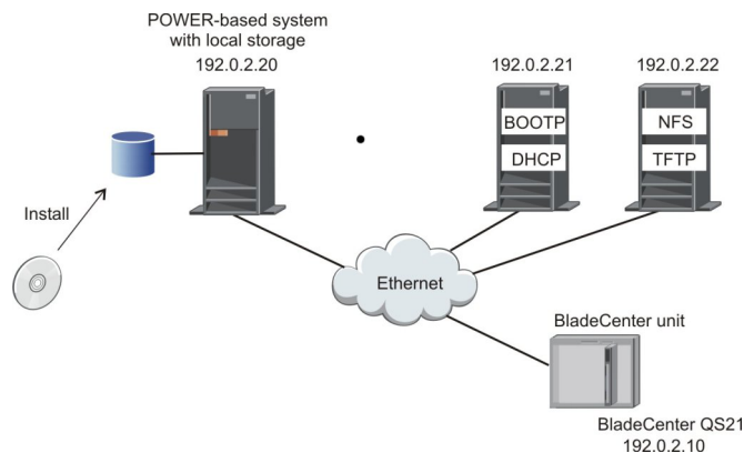
Figure 3. Sample setup with three systems
