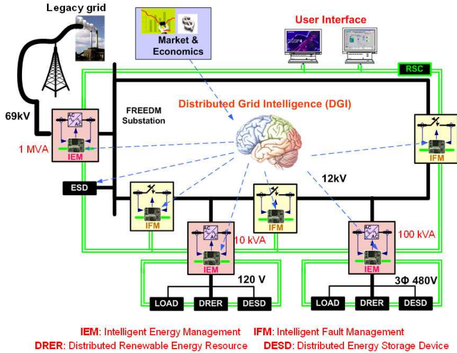
Figure 1. FREEDM System
