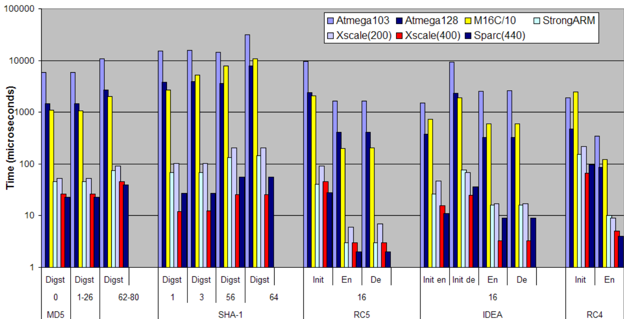
Figure 1: Execution times [μs] for algorithms, platforms and plaintext sizes [bytes]
